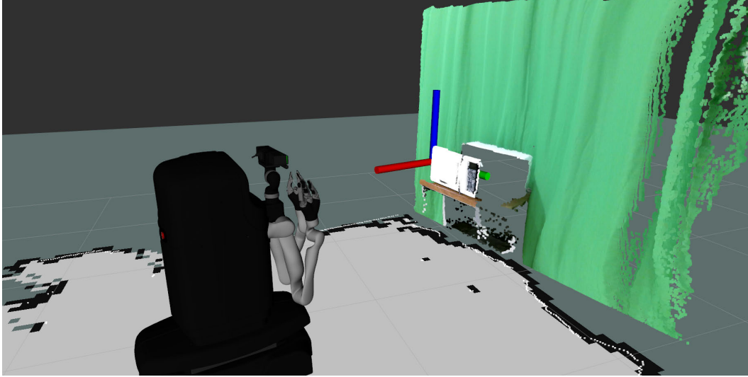
Figure 1: Kinematic model prediction for a novel object. Our model predicts the pose and state of a microwave’s hinge from a point cloud captured with a Kinect depth sensor.
