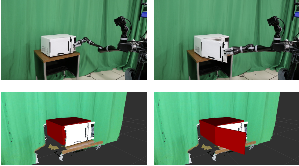
Figure 6: Novel object manipulation. Top: A MOVO robot manipulating a novel microwave using our system’s estimates of the object’s kinematics and geometry. Bottom: Rendered estimates of the object’s pose, geometry, and kinematic state before and after the manipulation.
