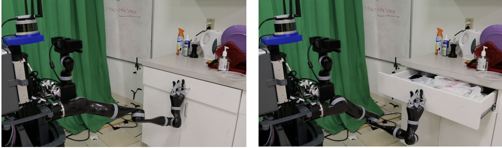
Figure 7: Novel object manipulation. A MOVO robot manipulating a novel drawer using a kinematic model estimated from a single depth image.
