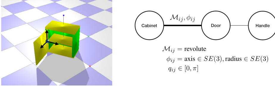
Figure 2: Kinematic Graph. A simulated object, annotated with the pose of its axis of rotation and corresponding kinematic graph. Our networks are trained to estimate model parameters \phi_{ij} and configuration q_{ij} for each joint of the object. We use the object’s categorization to select each model, \mathcal{M}_{ij} .
