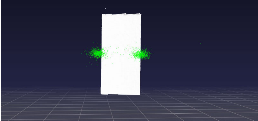
Figure 5: Model estimates under uncertainty. Samples drawn from the model of a cabinet’s hinge pose, accumulated over time and overlaid on a point cloud. With the door closed, it is challenging to discern whether the cabinet opens left or right. Accordingly, our model has assigned probability to both sides of the object.
