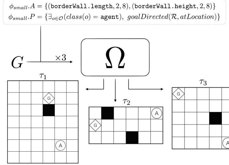
Figure 1: Three example tasks from the Grid World domain generated by \Omega .
